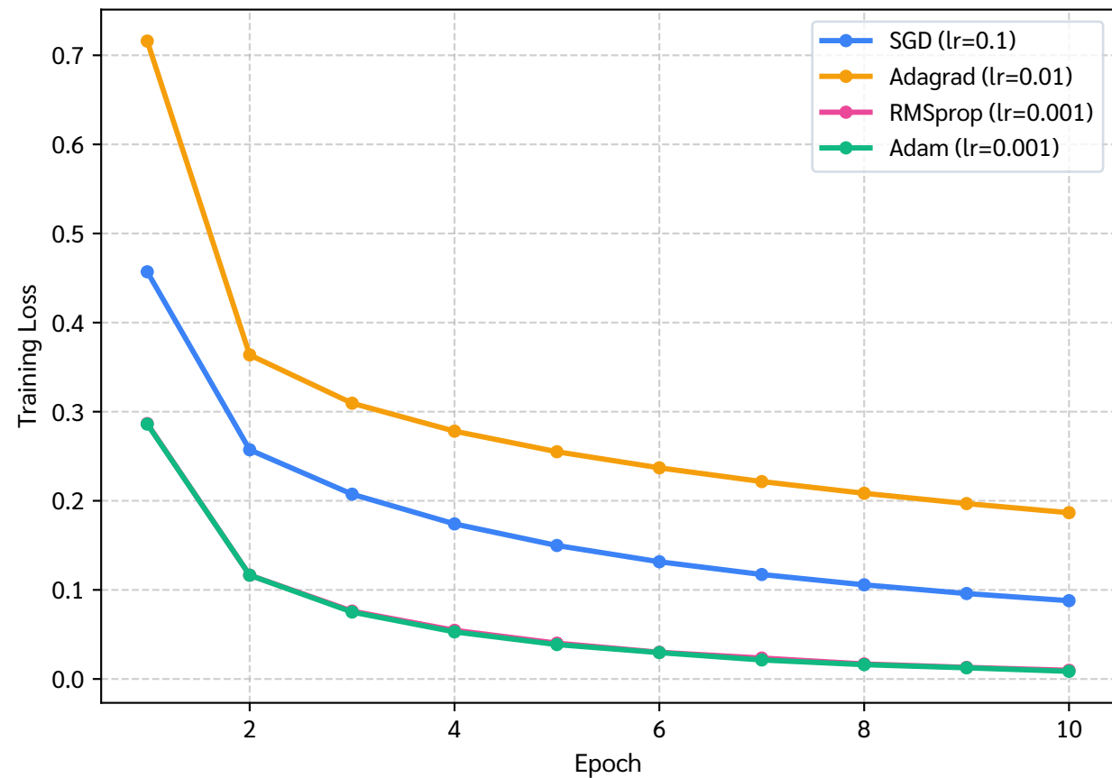
Training Loss Decay Across Optimizers
