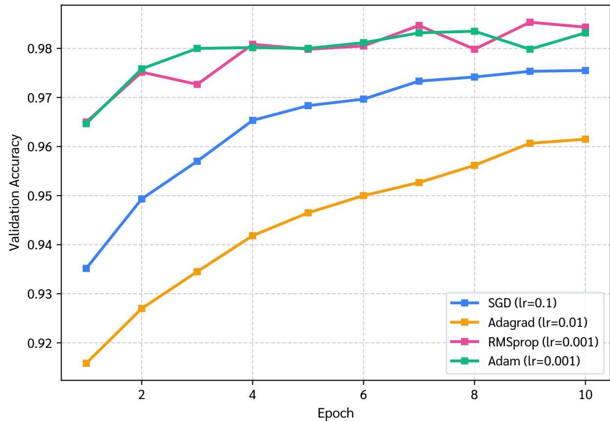
Validation Accuracy Dynamics Across Optimizers
